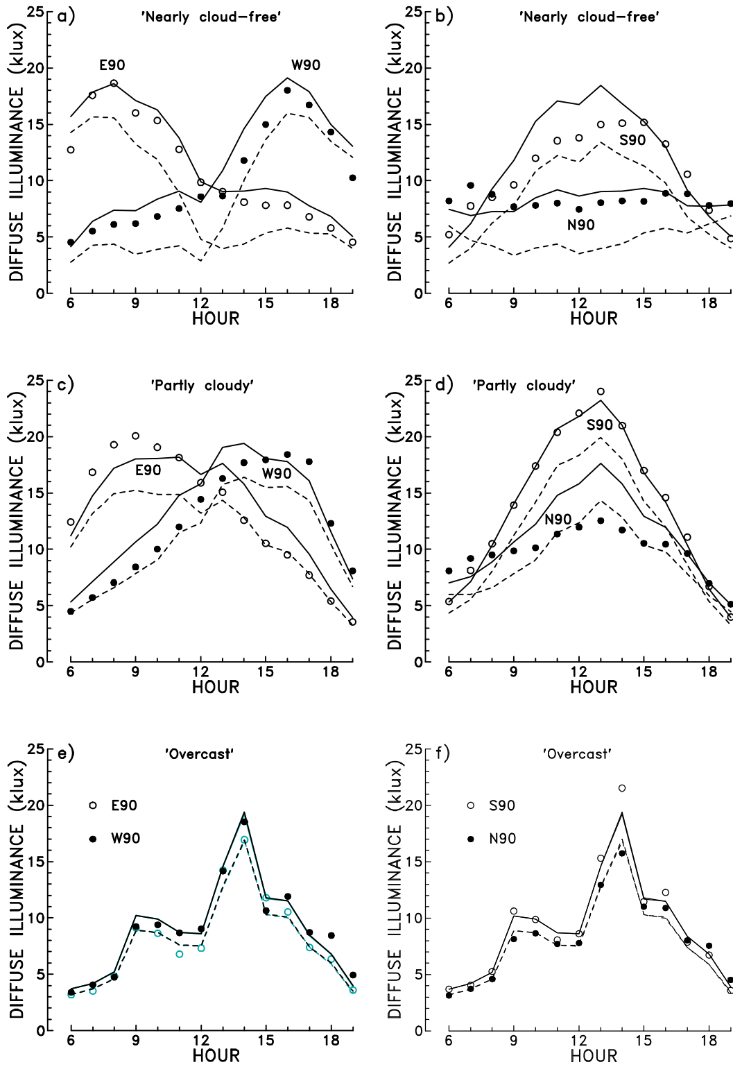
Fig.3 Vertical diffuse illuminance observed (dots) and modelled (curves) from horizontal beam and diffuse irradiances. Hourly mean values for "summer" days grouped as "nearly cloud-free", "partly cloudy", and "overcast" (see text). Fully drawn curves for foreground albedo = 0.1, and dashed curves for foreground albedo = 0.0.
