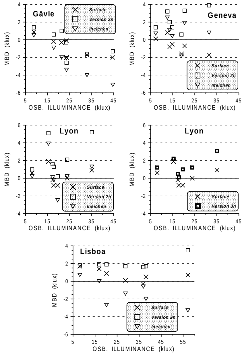
Fig. 6 Mean Bias Deviation (MBD=Modelled-Observed) vs observed illuminance of global, beam, and diffuse horizontal illuminance and illuminances on four vertical surfaces for the four stations. Illuminances are modelled from observed (surface), Heliosat Version 2n (V2n), Version 2n modified by Ineichen (Ineichen), and Heliosat Version 3n (V3n; for Lyon only) horizontal irradiances with foreground albedo A=0.1 .
