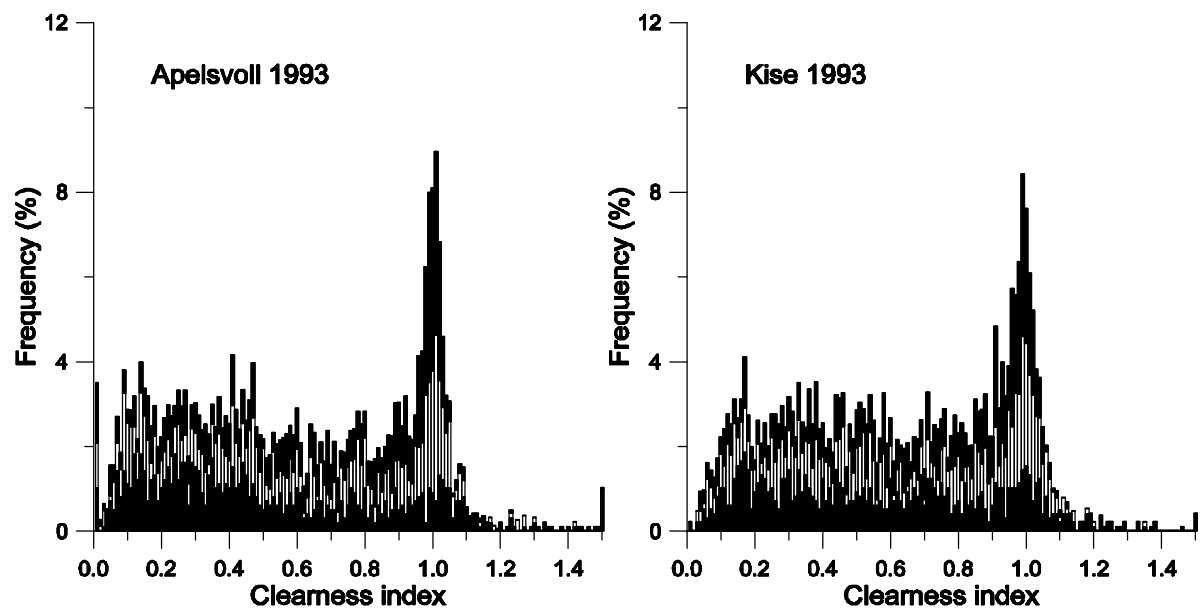
Fig.2a Distribution (percentage) of observed hourly clearness index within bins of width 0.01. Data from Apelsvoll and Kise during 1993 grouped into three solar elevation intervals: 10 - 20° (bottom), 20 - 30° (middle), and > 30° (top). See text for further details.
