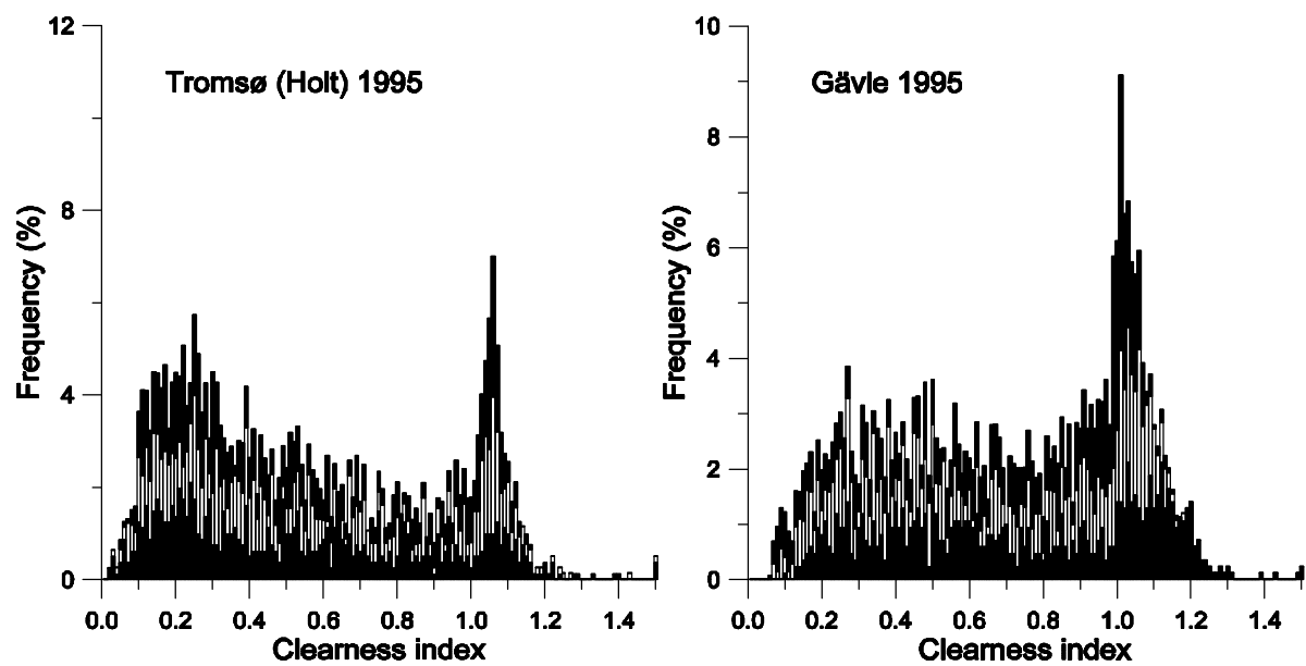
Fig.3e Same as Fig. 2a, but for Tromsø and Gävle 1995.
