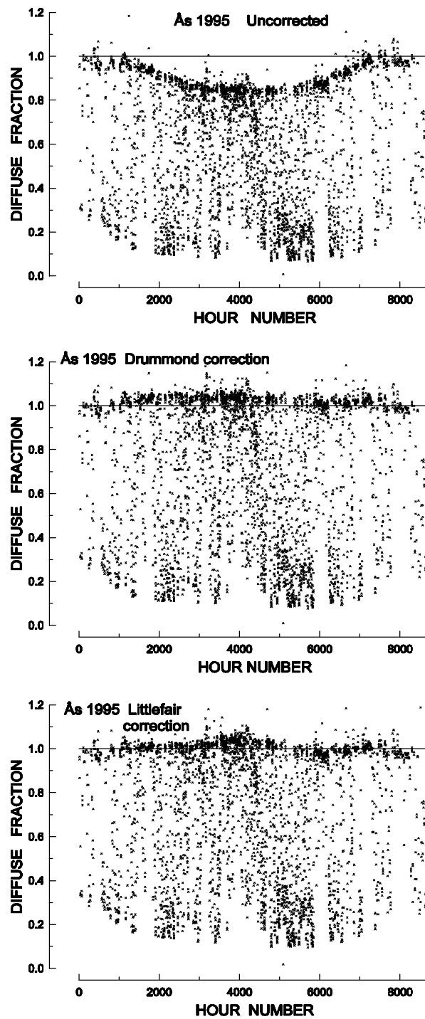
Fig.5 Top: Hourly diffuse fractions of global irradiance observed at Aas during 1995, with no shade ring correction applied. Middle: Same as above, but with the isotropic shade ring correction of Drummond [3] applied. Bottom: Same as above, but with the shade ring correction of Littlefair [4] applied.
