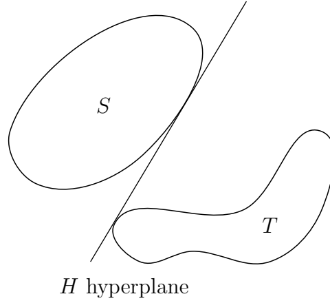
Figure 3.2: Separation
