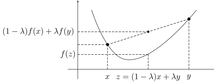
Figure 5.1: Convex function
