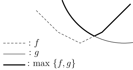
Figure 5.6: Maximum of convex functions
