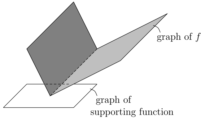
Figure 5.7: Supporting function
