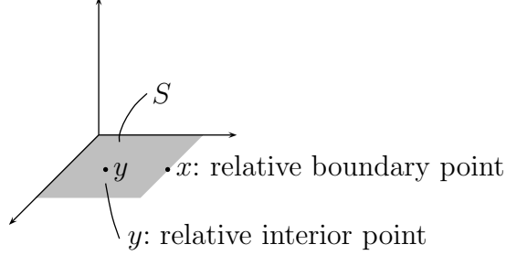
Figure 2.6: Relative topology
