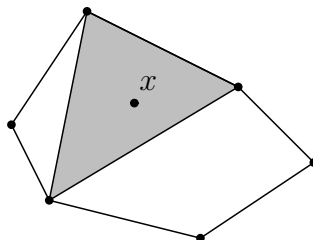
Figure 2.7: Carathéodory's theorem
