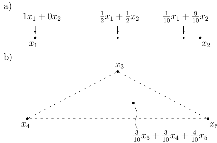
Figure 2.1: Convex combinations
