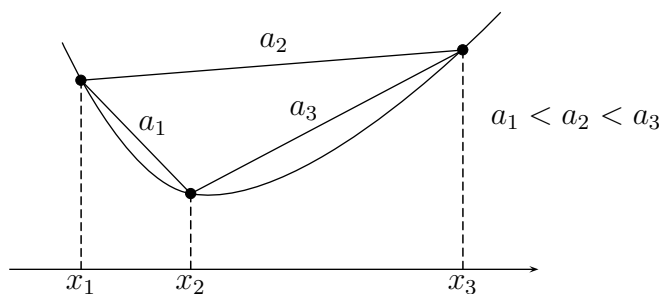
Figure 5.2: Increasing slopes
