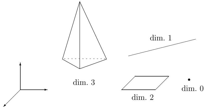
Figure 2.4: Dimensions
