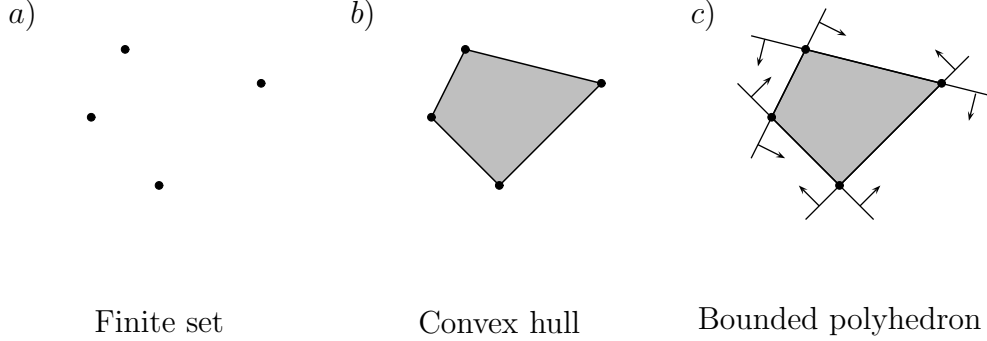
Figure 4.5: Polytope = bounded polyhedron
