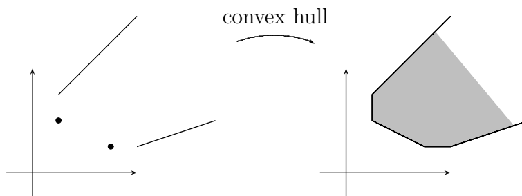
Figure 4.4: Minkowski's theorem, inner description
