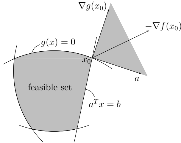
Figure 6.1: KKT conditions
