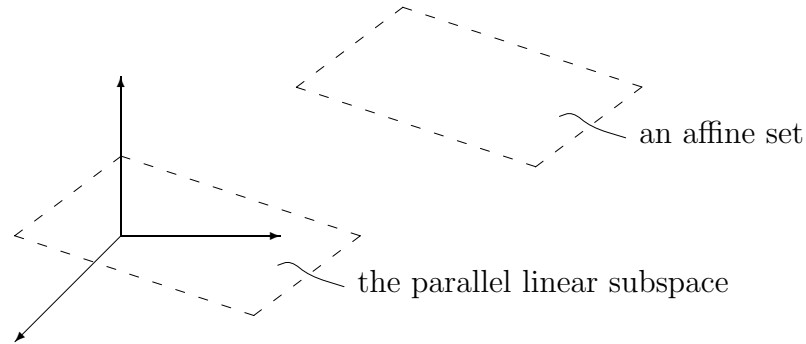
Figure 1.6: Affine set
