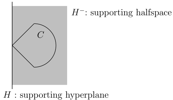
Figure 3.4: Supporting hyperplane and halfspace
