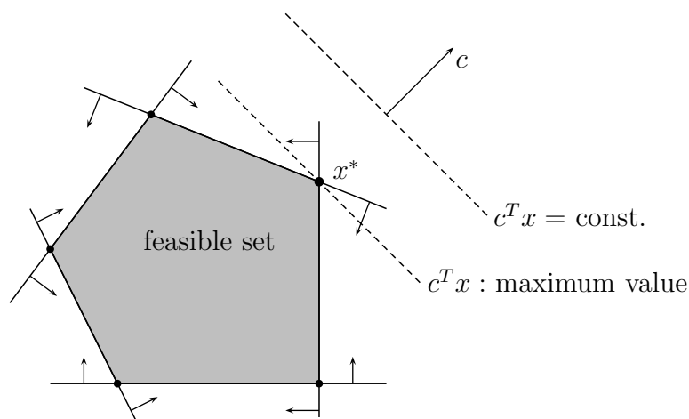
Figure 1.3: Linear programming
