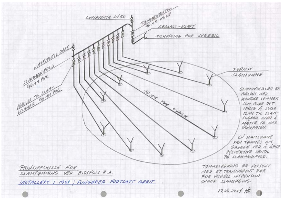
Figur 5.4 Prinsippet for slamtapping i en KMT-slammavskiller
