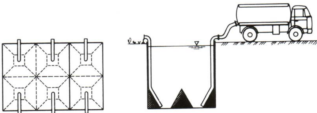
Figur 5.3 KMT slamavskiller
