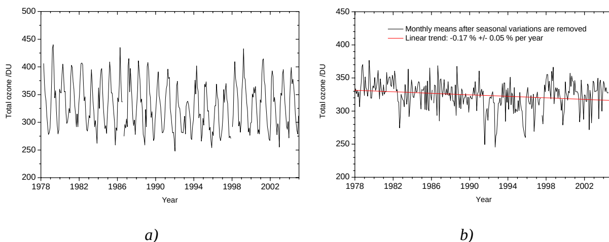
Figure 6a: Time series of monthly mean total ozone in Oslo.
