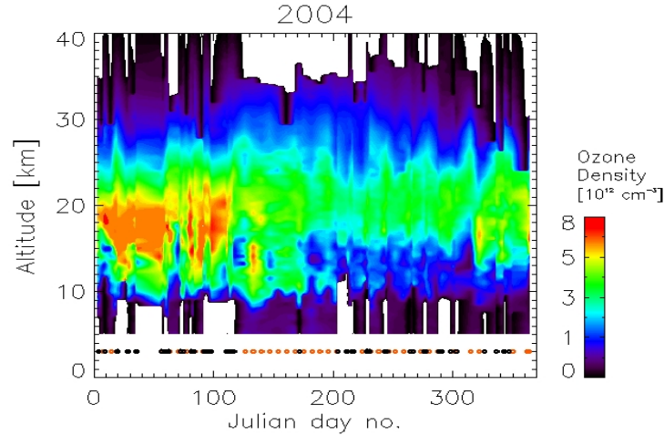
Figure 3: Ozone profiles measured by the ALOMAR ozone lidar and ozone sondes launched in Sodankylä, Finland, in 2004. The black diamonds at the bottom of the plot mark the times when lidar measurements were performed, while the red diamonds mark days where data from ozone sondes launched from Sodankylä were used. Between the individual measurements the data were linearly interpolated and smoothed with a one-week median filter.
