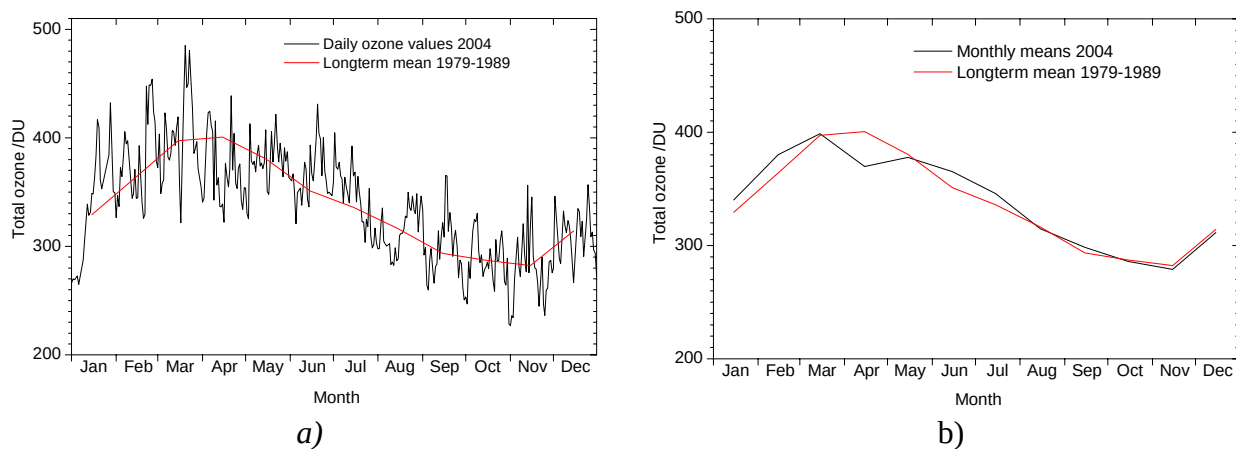
Figure 1a): Daily total ozone values measured at the University of Oslo in 2004. The red curve shows the long-term monthly mean values from 1979-1989.
