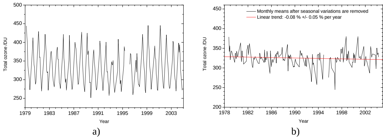
Figure 8 a): Time series of monthly mean total ozone at Andøya.
