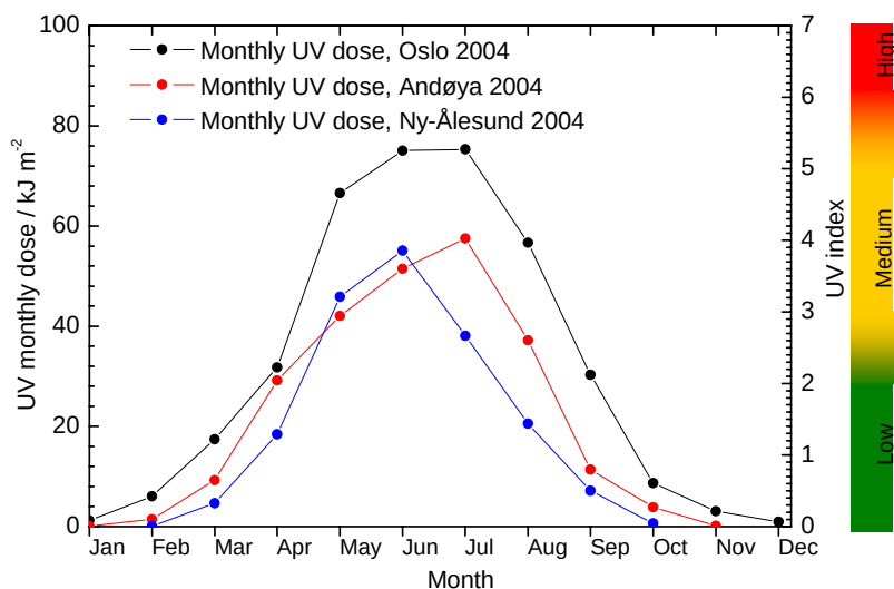
Figure 12: Monthly integrated UV doses in 2004 measured with the GUV instruments located in Oslo and at Andøya.
