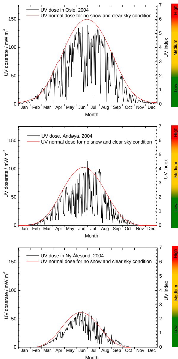
Figure 11: Hourly averaged UV dose rate measured at noon (between 10:30 and 11:30 GMT) at a) Oslo, b) Andøya, c) Ny-Ålesund
