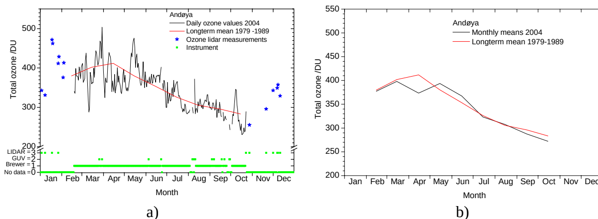
Figure 2a): Daily total ozone values measured at ALOMAR, Andøya in 2004 by the Brewer, GUV and LIDAR instruments. The use of the different instruments is shown in the lower panel of Figure 2a). The red line shows the long-term monthly mean values from 1979-1989.
