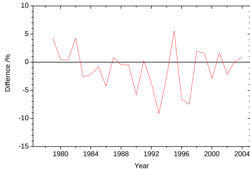
Figure 9: Percentage difference between yearly mean total ozone at Andøya and the long-term yearly mean for 1979 – 1989 for the months March - September
