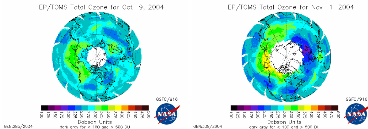
Figure 5: TOMS data of daily total ozone values for 9 October, 1 November 2004.
