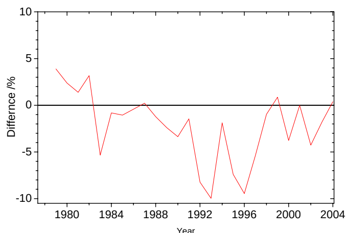
Figure 7: Percentage difference between yearly mean total ozone in Oslo and the long-term yearly mean for 1979-2001.
