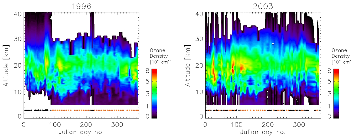
Figure 4: Ozone profiles measured by the ALOMAR ozone lidar and ozone sondes launched in Sodankylä, Finland, in 1996 (left panel) and 2003 (right panel) [analog to Figure 1].
