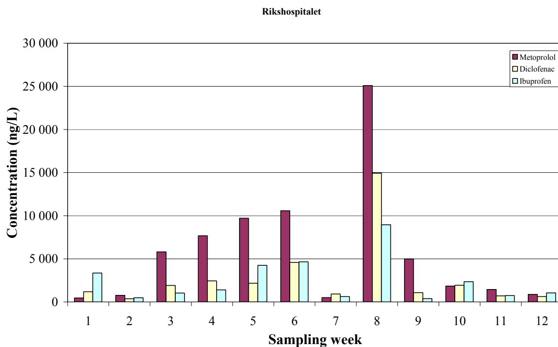
Figure 12 Concentration of metoprolol, diclofenac and ibuprofen in Rikshospitalet effluent samples
