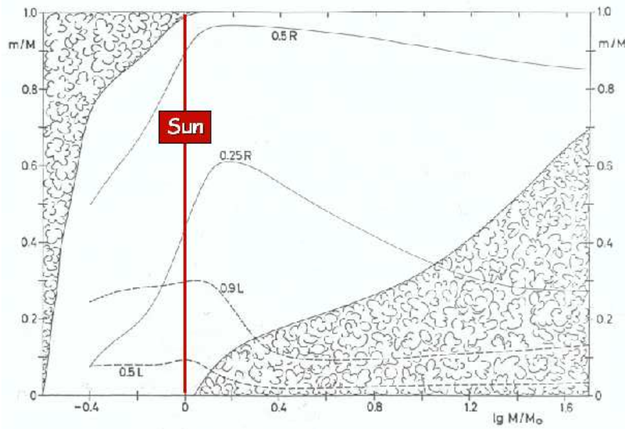
Figure 7.1.: In the shadowed regions convection is important for main sequence stars, the x axis labels the total mass of the stars, x = \log(M/M_\odot) , while the y axis labels the position in the star, y = M(r)/M .
