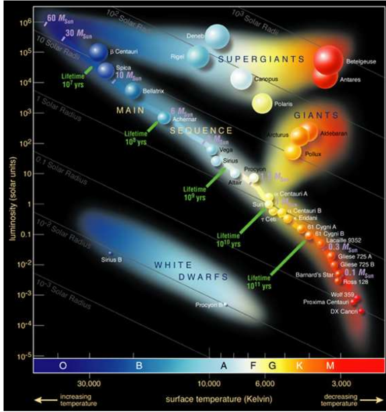
Figure 2.2.: A Hertzsprung-Russell diagram. The position of a star along the main-sequence defines uniquely all important stellar parameters: Mass, radius, temperature, lifetime.
