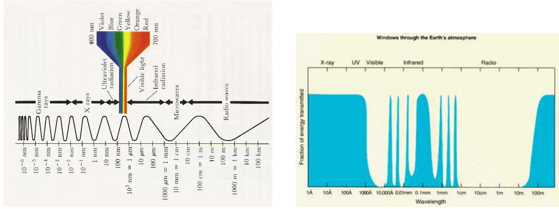
Figure 1.1.: Left: The electromagnetic spectrum. Right: The transmission of the Earth's atmosphere as function of the wavelength.
