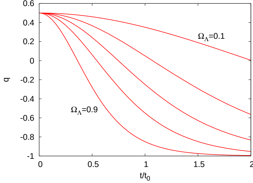
Figure 15.3.: The deceleration parameter q as function of t/t_0 for the \Lambda CDM model and various values for \Omega_\Lambda (0.1, 0.3, 0.5, 0.7 and 0.9 from the top to the bottom).
