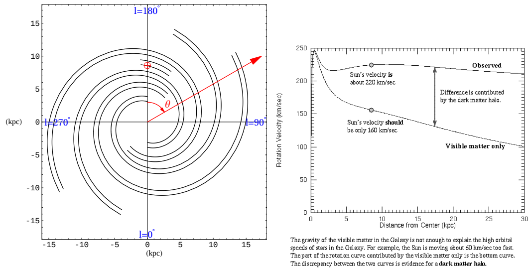
Figure 13.1.: Left: Schematic view of the spiral structure of the Milky Way; the position of the Sun is marked by a red dot. Right: Rotation curve of the Milky Way.
