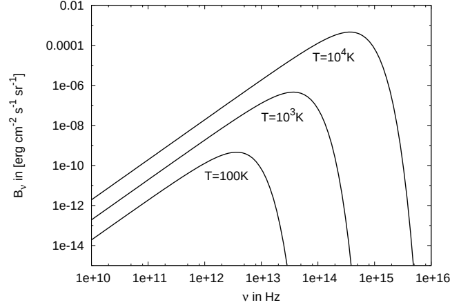
Figure 1.4.: The Planck distribution B_\nu as function of the frequency \nu for three different temperatures.
