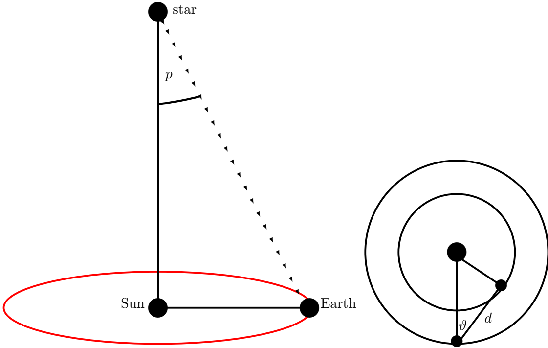
Figure 1.6.: Measurement of the trigonometric parallax. Left: The apparent movement of a nearby star during a year: Half of this angular difference is called the parallax angle or simply the parallax p . Right: Indirect determination of the Earth-Sun distance.
