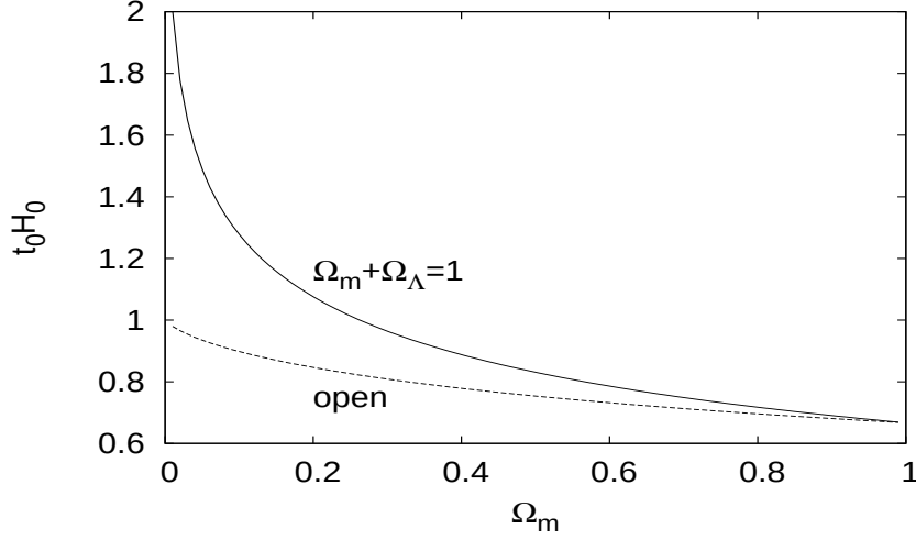
Figure 15.2.: The product t_0 H_0 for an open universe containing only matter and for a flat cosmological model with \Omega_\Lambda + \Omega_m = 1 .
