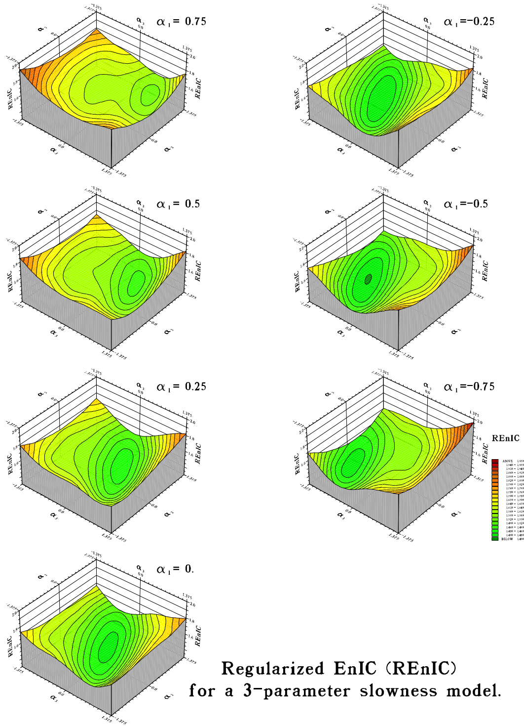
Figure 4: Regularized EnIC (REnIC) for a 3-parameter slowness model
