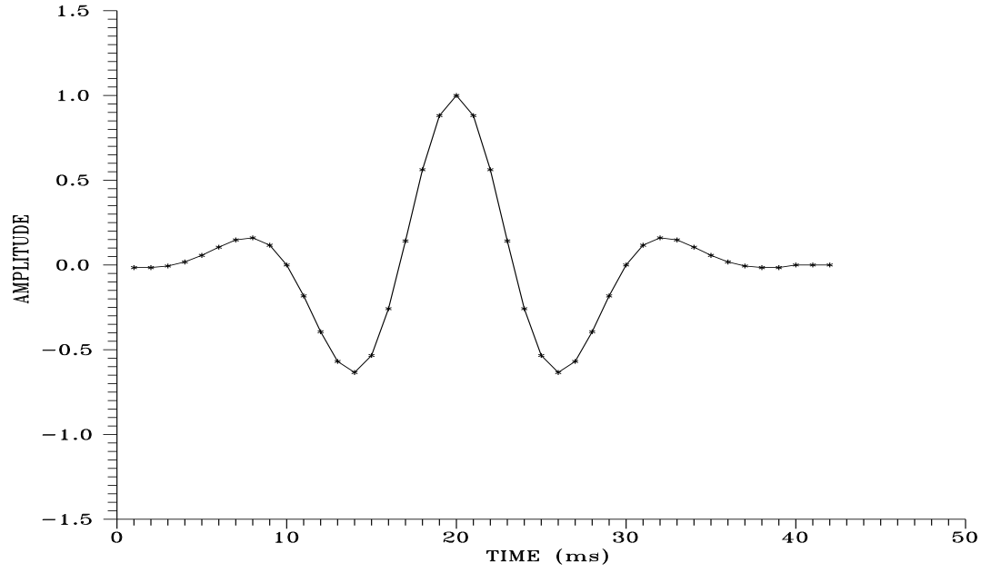
Figure 2: Source wavelet.
