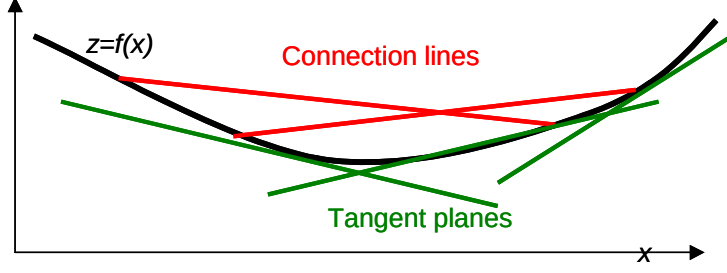
Figure 4: A useful mental image of a convex function: Connecting line segments above, and tangent planes below the graph!
