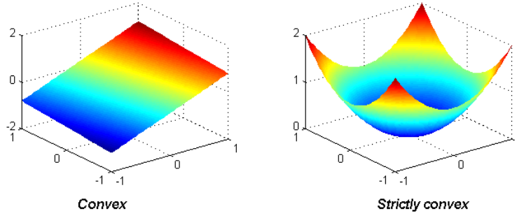
Figure 3: Simple examples of graphs of convex and strictly convex functions (to be used only as a mental image!).
