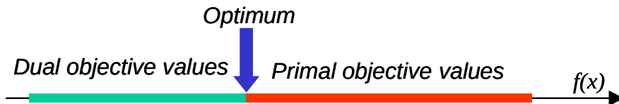
Figure 1: The objective values for the dual are to the left of the values for the primal. The maximum of the dual and the minimum of the primal objectives are the same.
