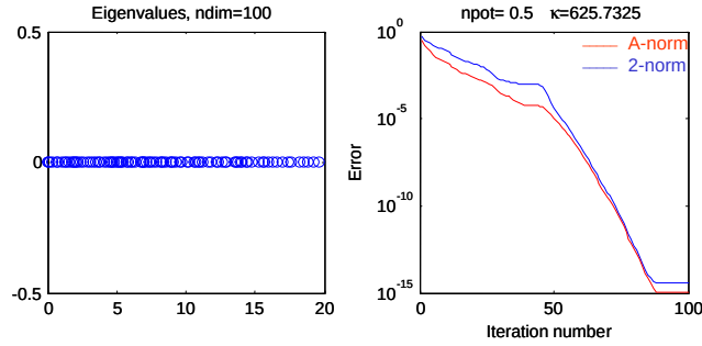
Figure 3: Medium conditioned matrix.
