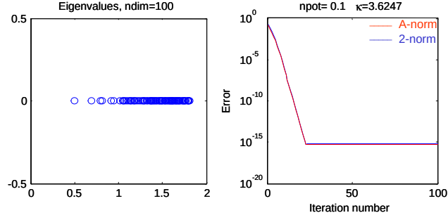
Figure 2: Well-conditioned matrix. Fast convergence.
