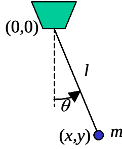
Figure 1: Simple pendulum.
