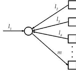
Figure 13.2: Processing at the variable nodes
