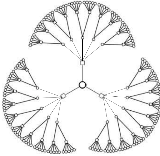
Figure 13.1: Computation graph of depth 4. All nodes appearing in the graph must be distinct in order for the independence assumption to hold.
