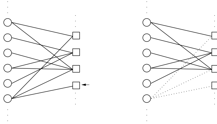
Figure 13.4: Iterative decoding for BEC. In each iteration, first find a check node of degree 1 (left), then remove all the edges emanating from the neighboring variable node (right)
