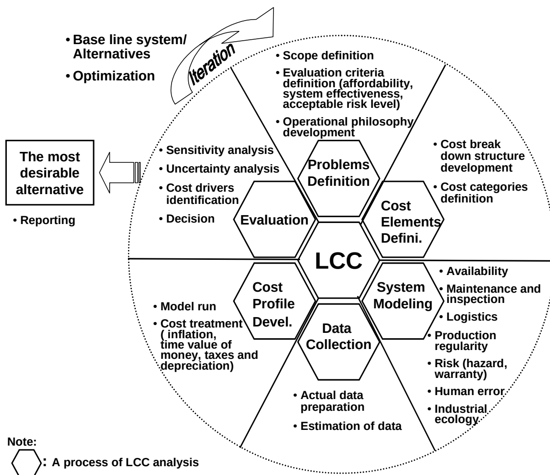
Figure 5-2: A LCC concept map (The six basic processes and sub-activities)
