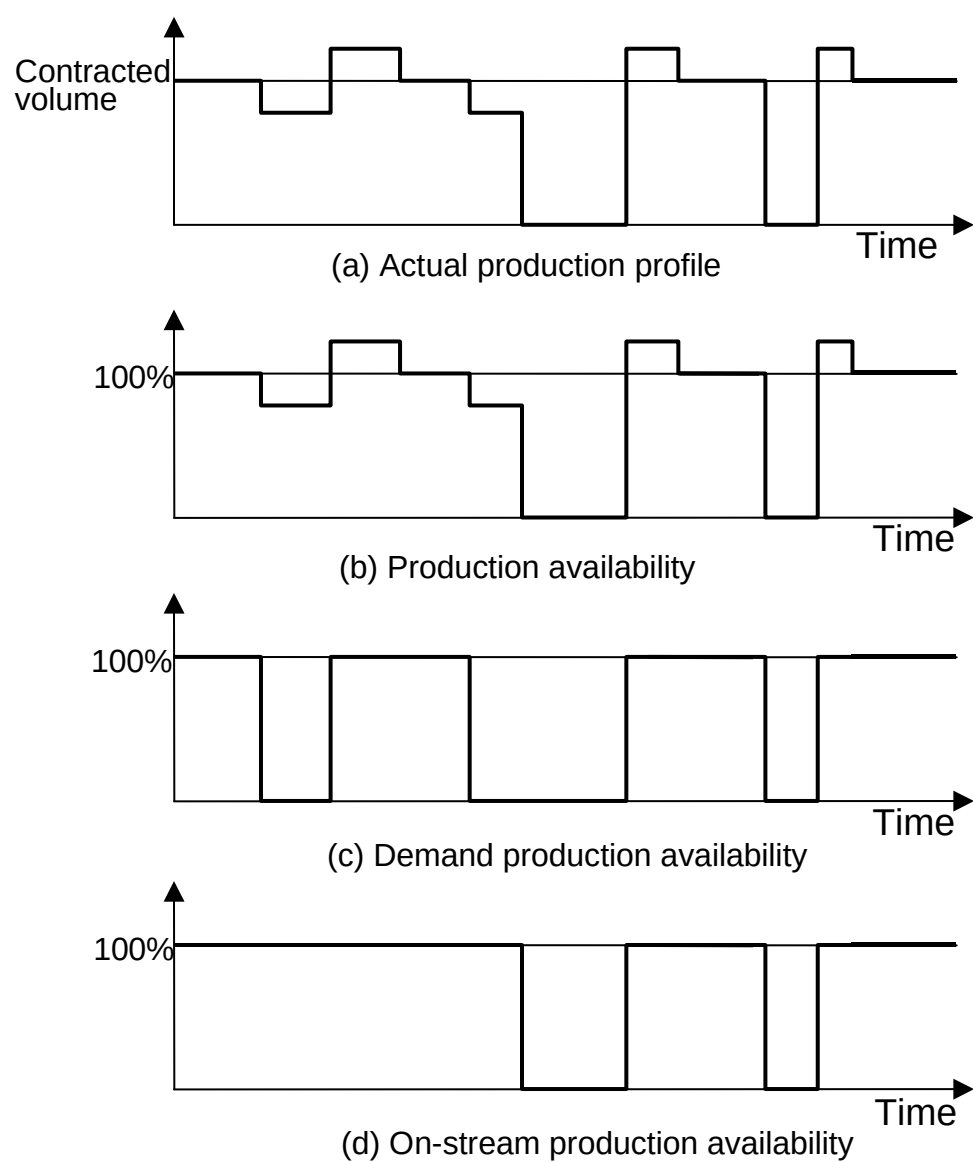
Figure 5-8: Illustration of different “production availability” measures
