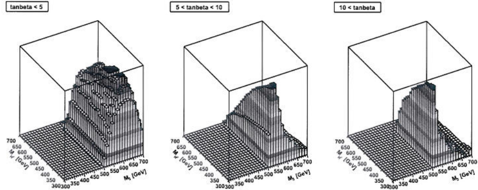
Figure 3: Distribution of M_3 -values for M_1 = 100 GeV, M_2 = 300 GeV and \mu = 500 GeV. Three slices of \tan \beta -values are shown, increasing to the right.
